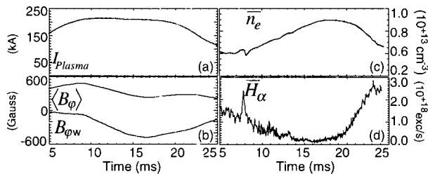
FIG. 6. (a) Plasma current, (b) average toroidal magnetic field and toroidal field measured at the wall, (c) line-averaged electron density measured through a central chord, and (d) the line-averaged H_\alpha excitation rate for a high-confinement plasma discharge.
