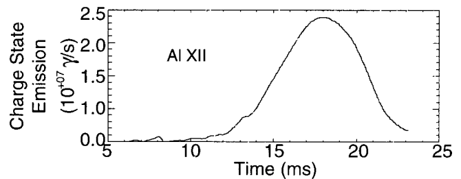
FIG. 7. Line intensity of the Al XII He-like 1s^2-1s2p transition.
